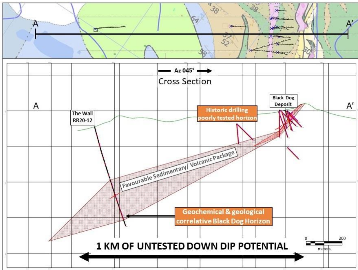
Cross section of The Wall target demonstrates favourable geology down dip from the Black Dog Deposit. There is significant open ground to be evaluated and other historic drilling may not have tested down dip potential.
